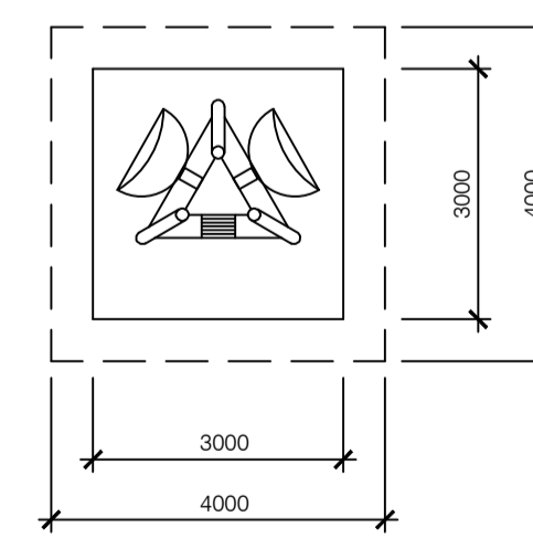
PLAN SCALE 1:100
