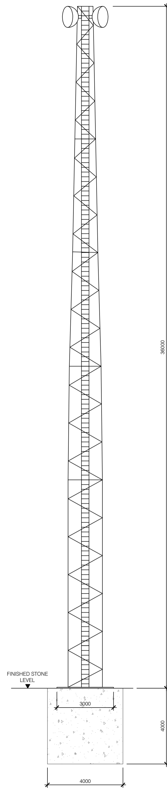
FRONT ELEVATION SCALE 1:100
