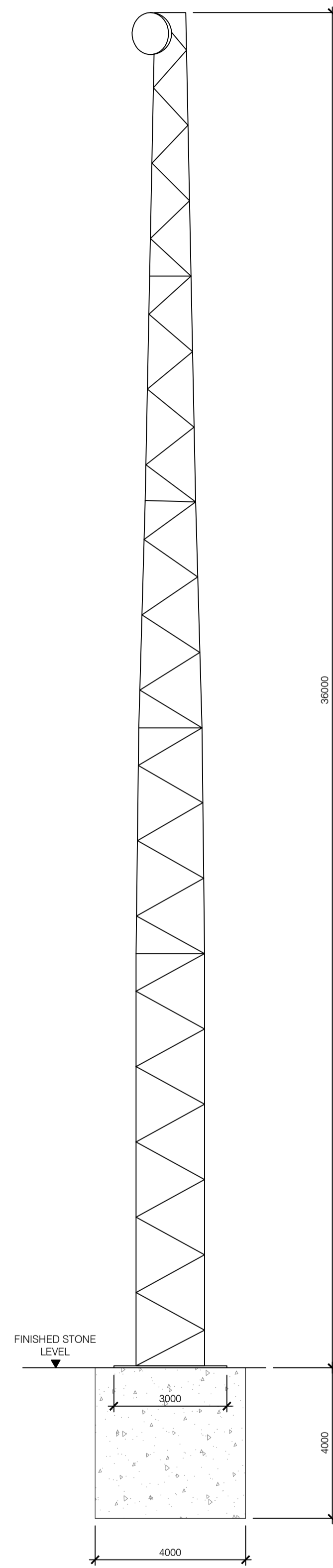
SIDE ELEVATION SCALE 1:100
